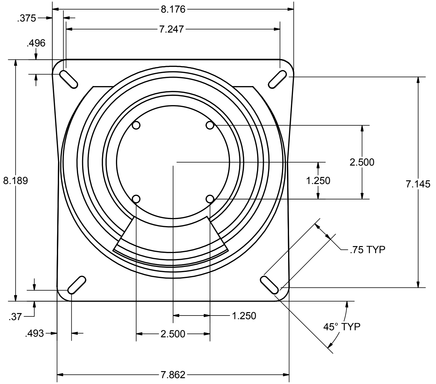
BOTTOM VIEW
